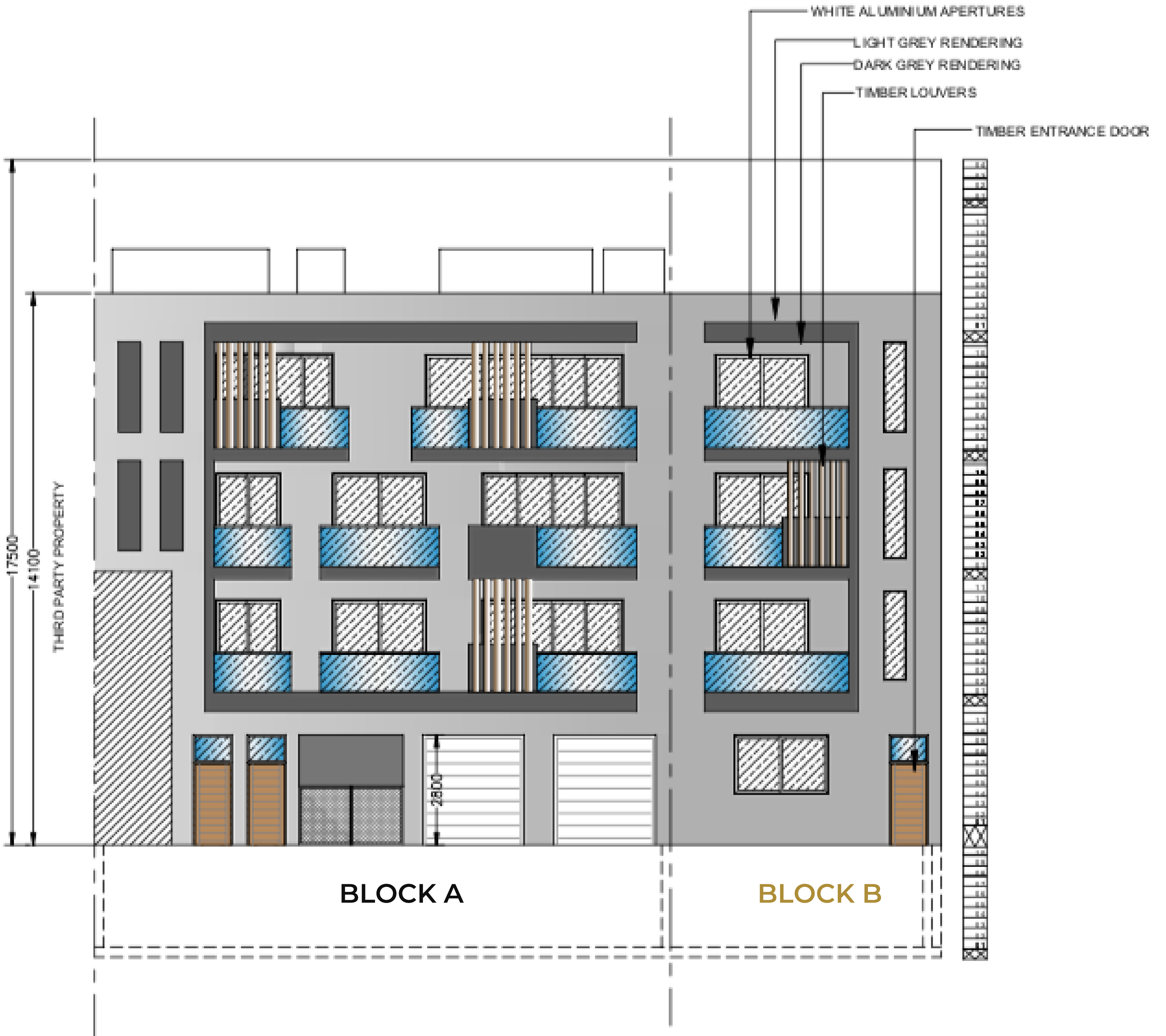
ELEVATION A SCALE 1:100
