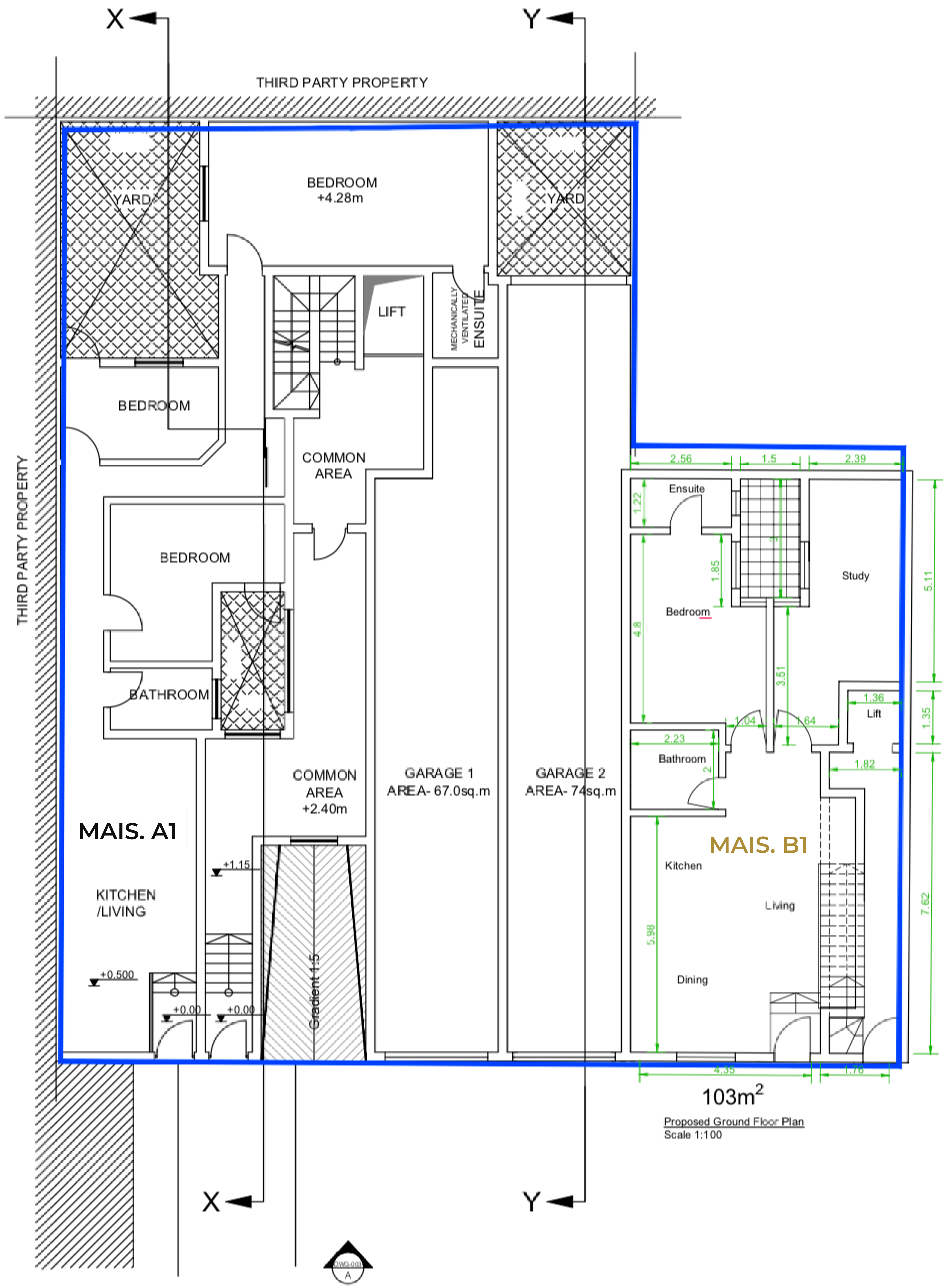
PROPOSED GROUND FLOOR SCALE 1:100
