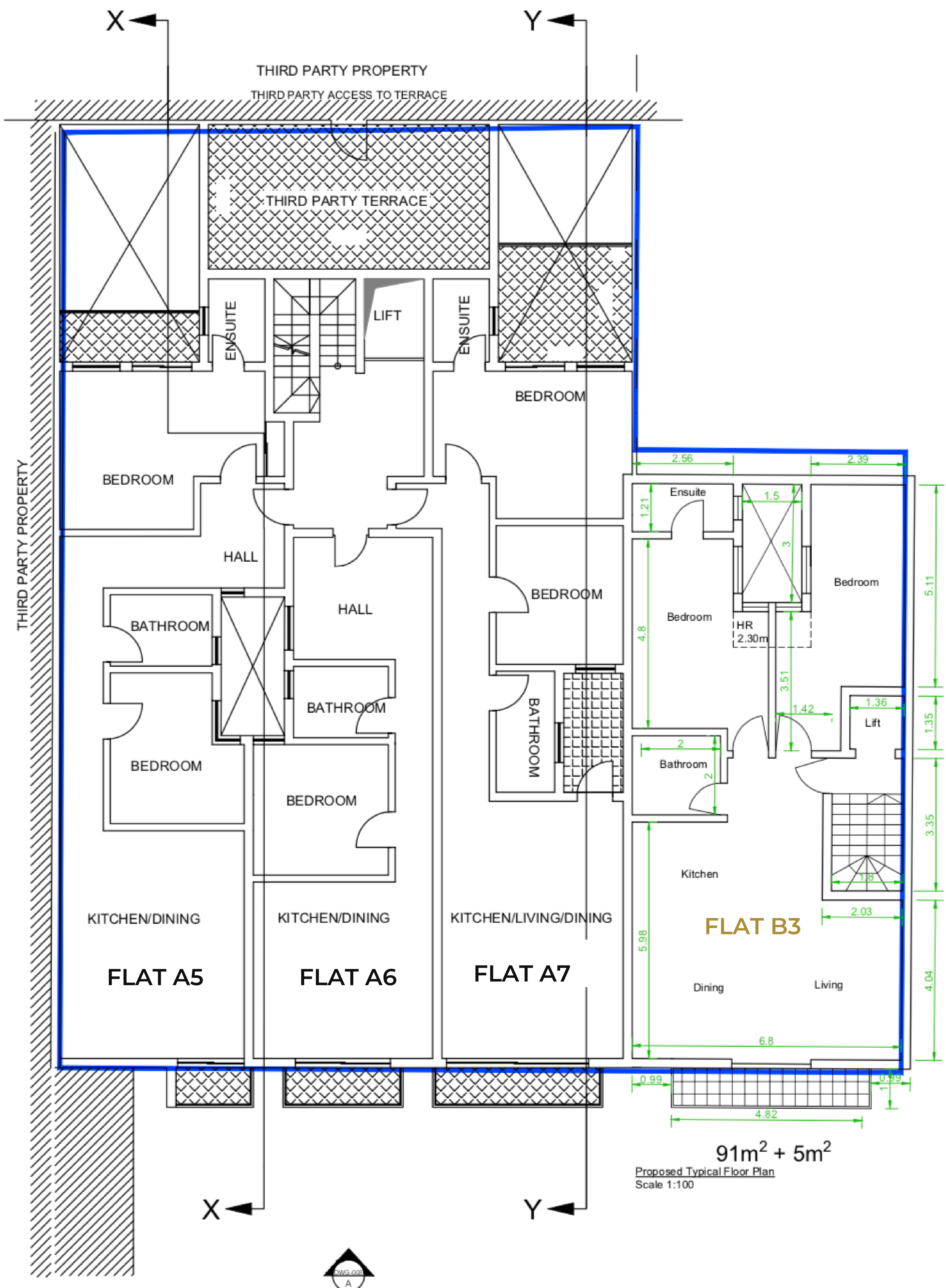
PROPOSED SECOND FLOOR PLAN SCALE 1:100
