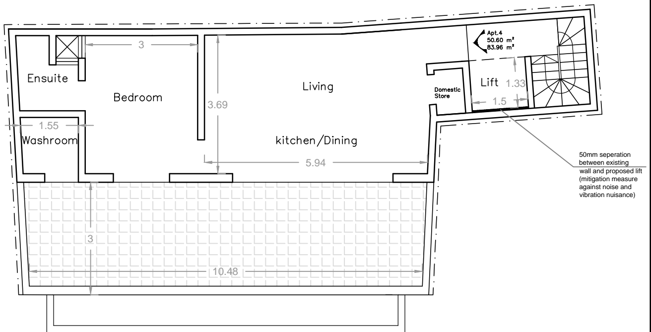
Proposed Receded Floor Plan scale 1:100
