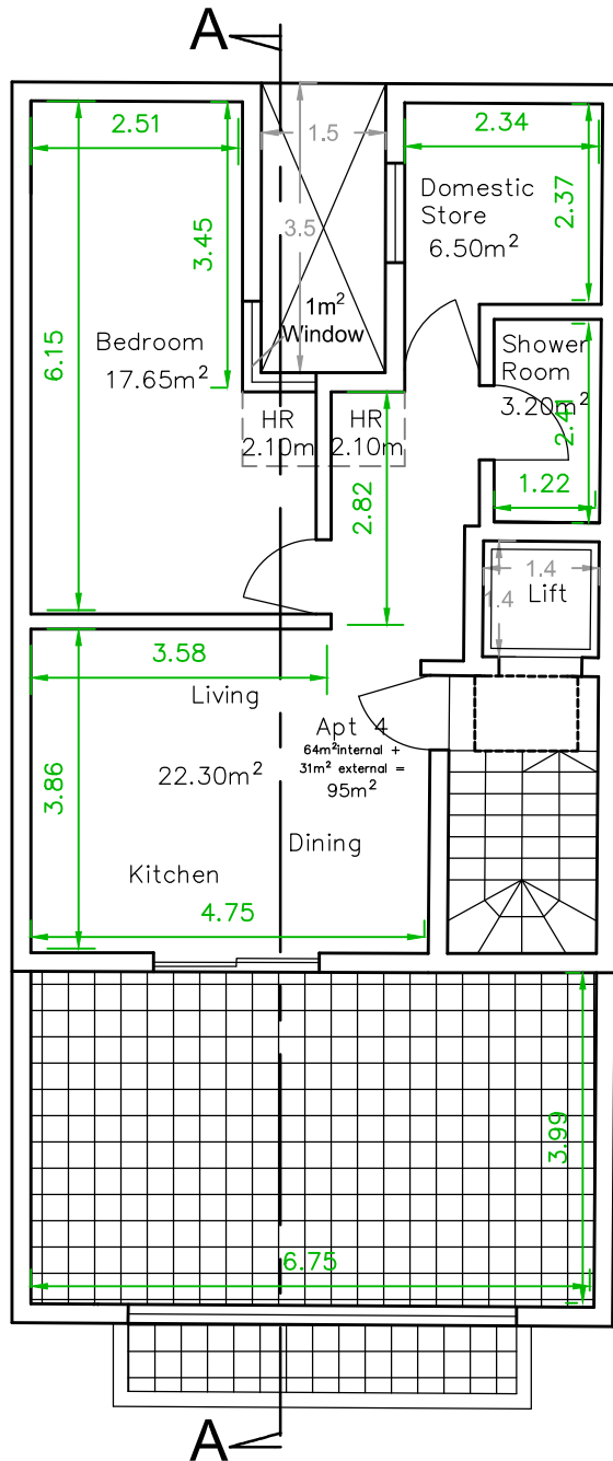
Proposed Receded Floor Plan Scale 1:100
